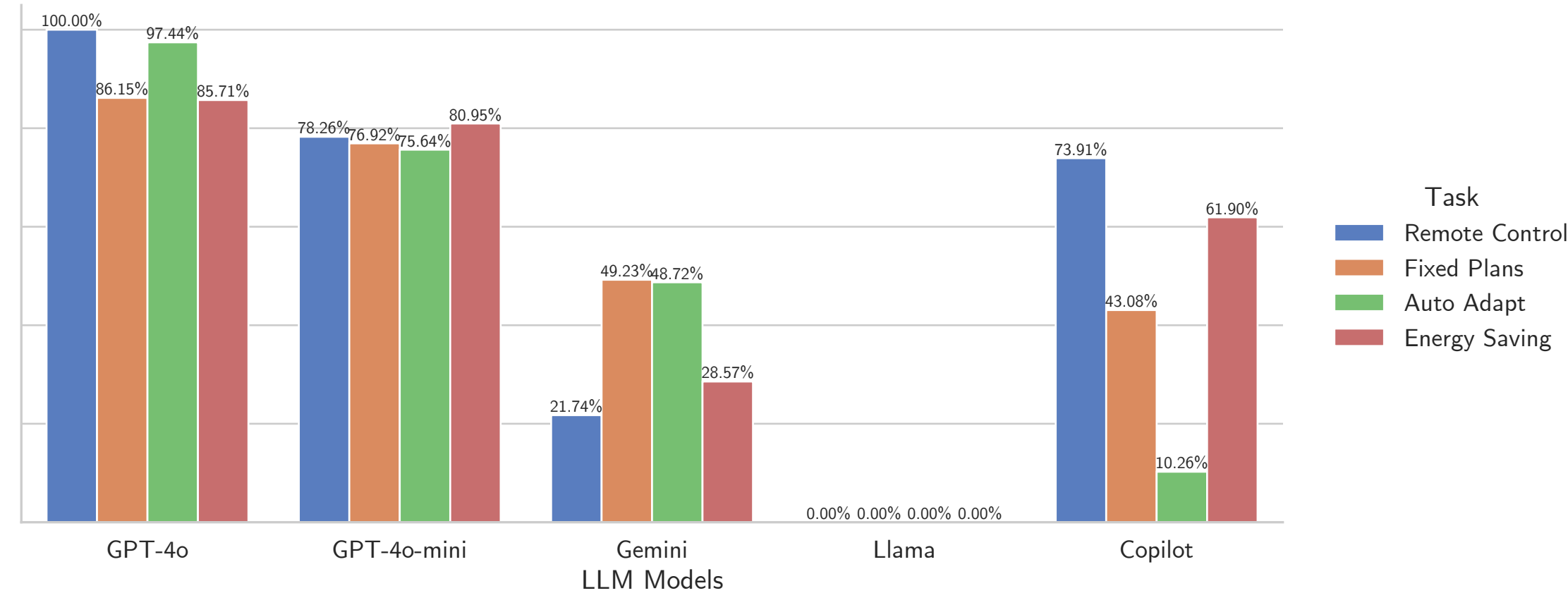
COMPILEABLE RATE by Task in English
