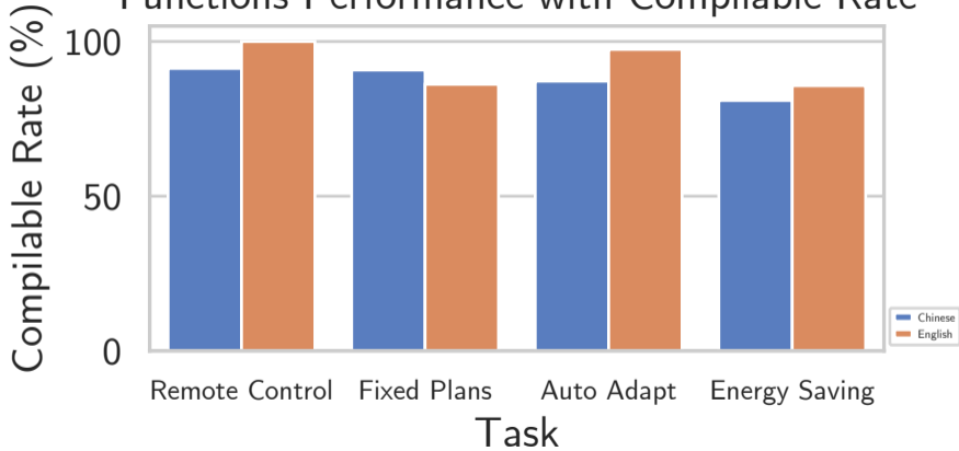
Functions Performance with Compilable Rate
