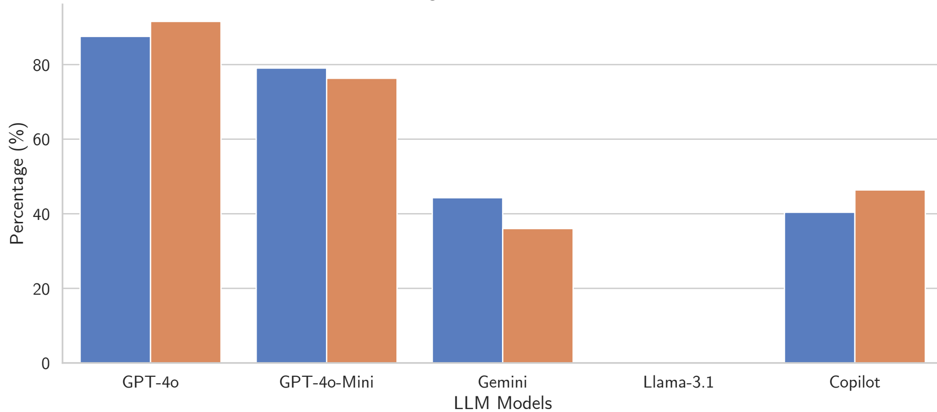
Average COMPILABLE RATE
