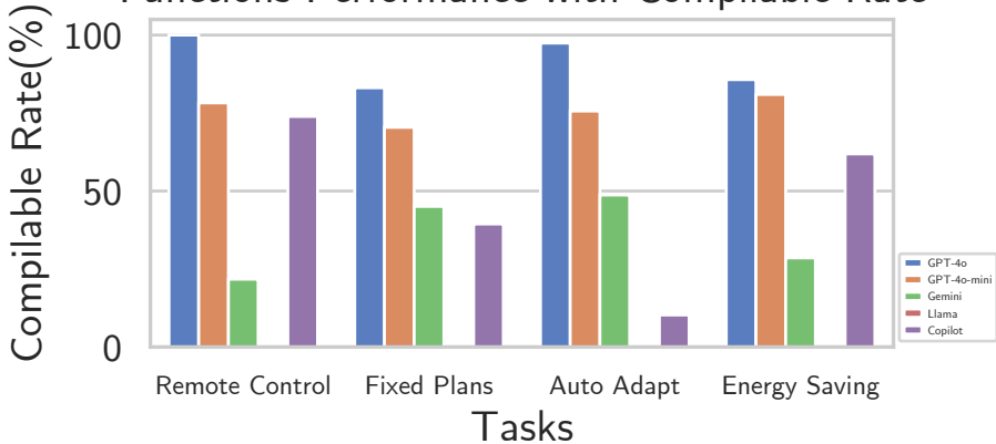
Functions Performance with Compilable Rate
