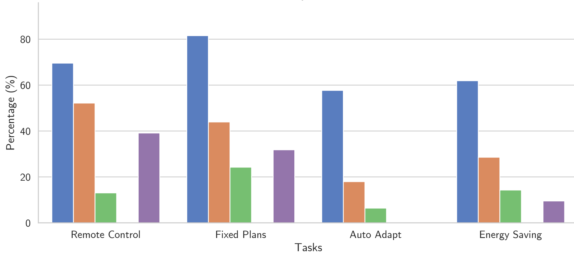
PASS RATE by Task in Chinese
