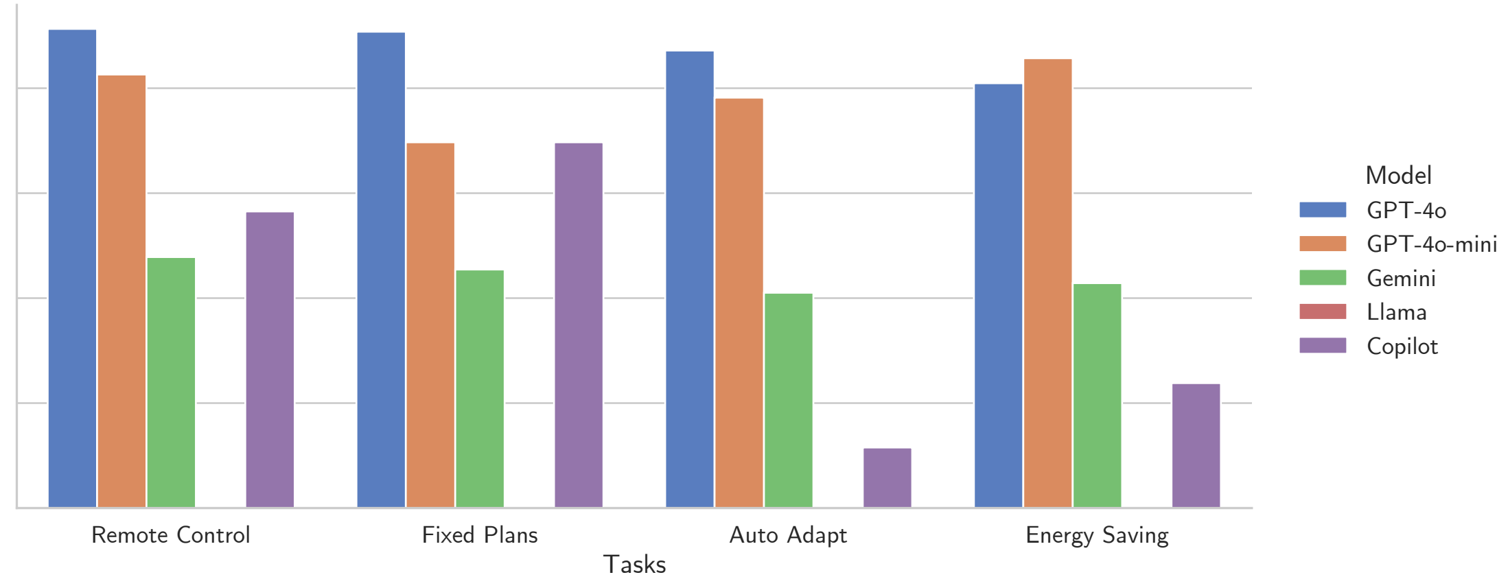
COMPILEABLE RATE by Task in Chinese
