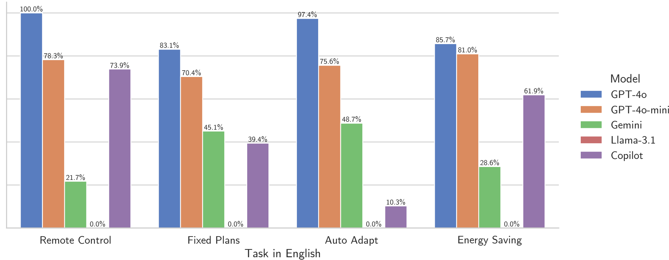
COMPILABLE RATE by Task in English
