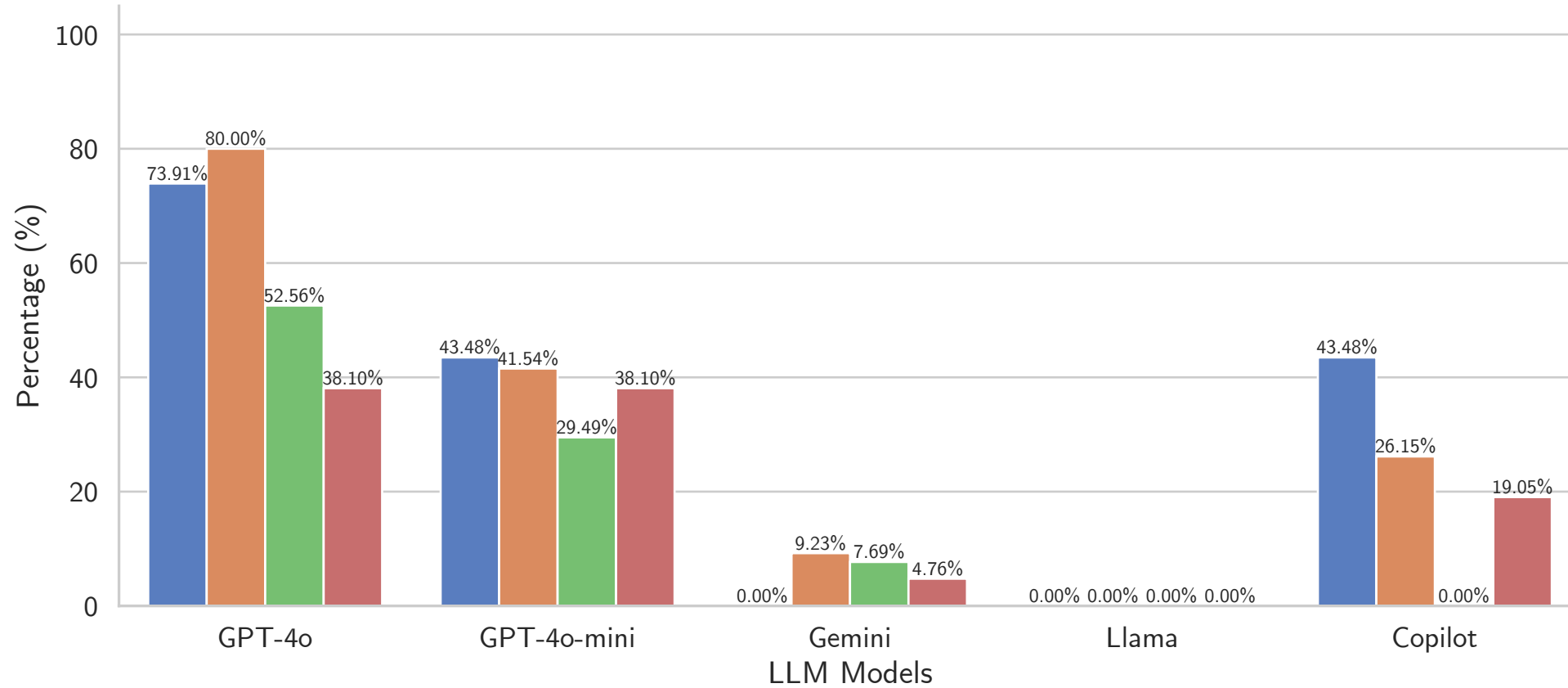
PASS RATE by Task in English
