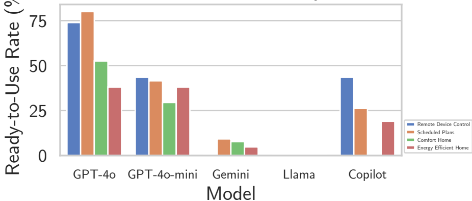
Functions Performance with Ready-to-Use Rate
