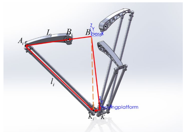
图 1 空间机构向量闭环关系构建 Fig.1 Construction of vector loop-closure relations for spatial mechanisms
