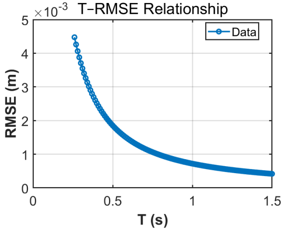
图 9 末端轨迹跟踪误差随运动周期变化关系曲线 Fig.9 Effect of Motion Period on End-Effector Tracking Accuracy
