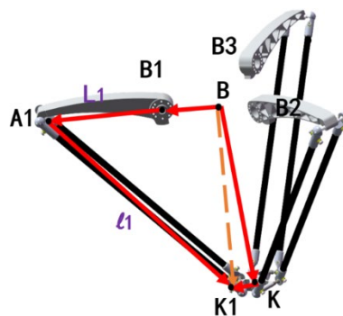
图 1 空间机构向量闭环关系构建 Fig.1 Construction of vector loop-closure relations for spatial mechanisms
