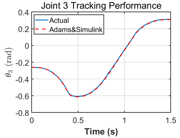
(c) 关节 3 (c) Joint 3
