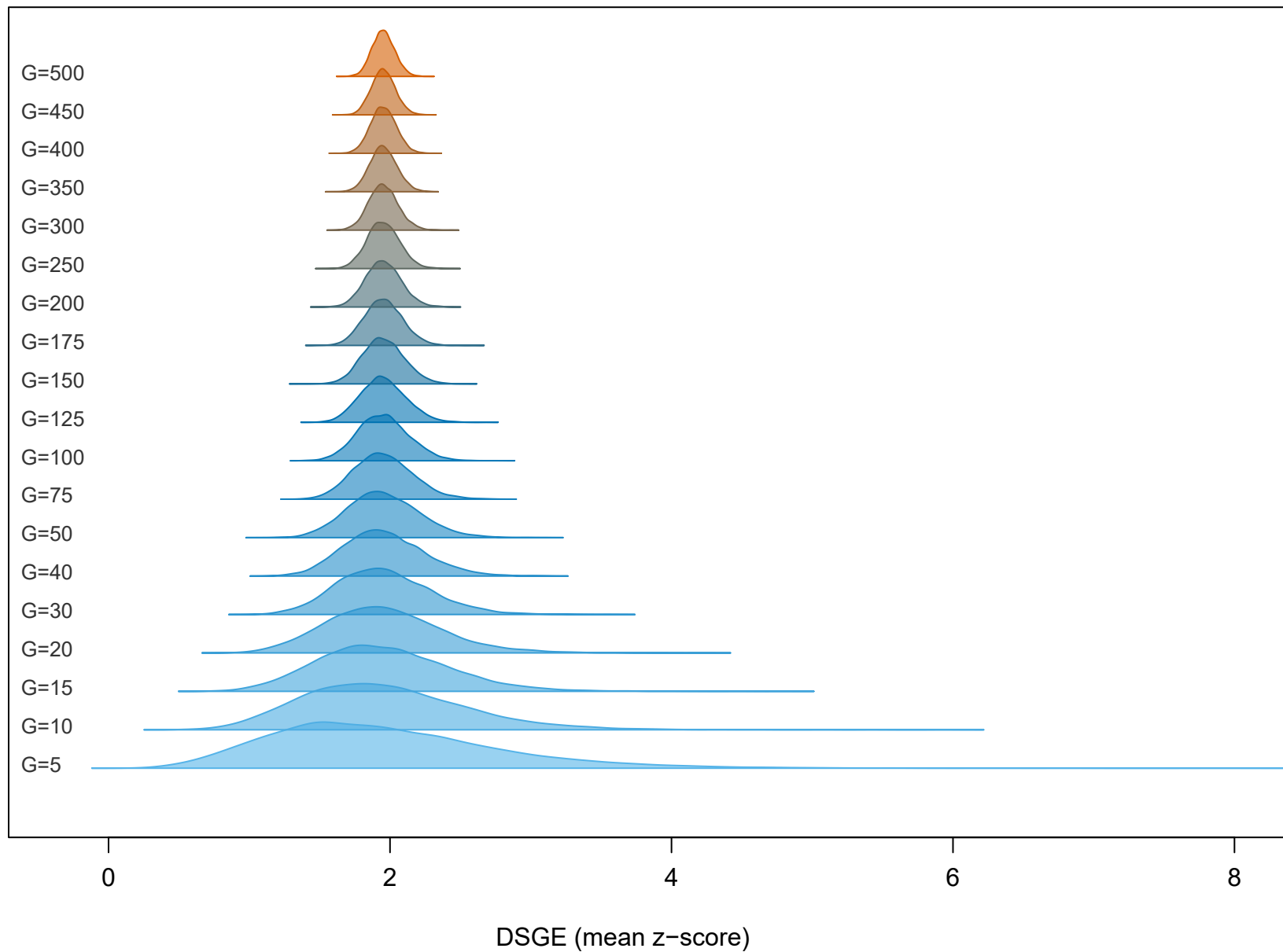
Null Distribution Ridgeline (Size 5 to 500)
