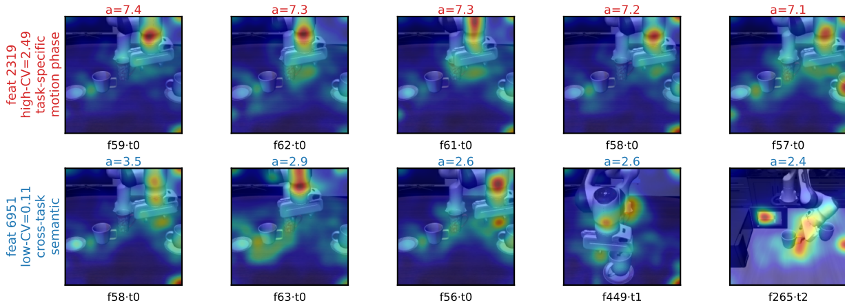
(b) top-activating LIBERO frames per feature (overlay = |\nabla \text{feat} \cdot \text{image}| )
