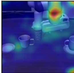
feat 2319 high-CV=2.49 task-specific motion phase
