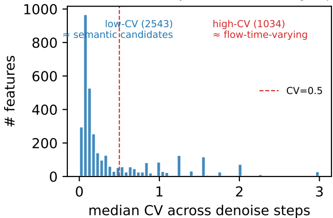
Aim 3: feature stability across flow-matching steps
