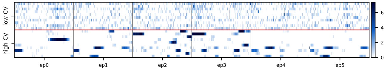
(d) activation heatmap of top-10 low-CV / top-10 high-CV features (rows) across episode-sorted frames (cols)
