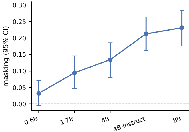
(a) TriviaQA, C-line, k=1
