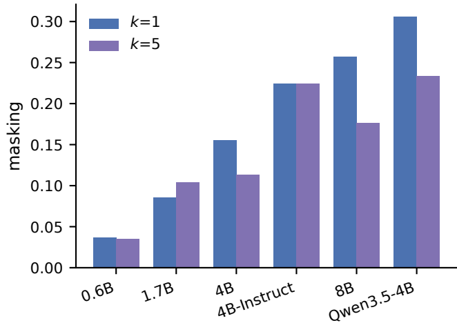
(b) TriviaQA, B-line, six models
