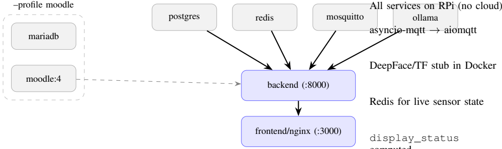
Fig. 16. Docker Compose service dependency graph.
