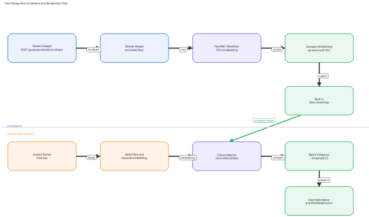
Fig. 20. Face recognition enrollment and recognition flow.
