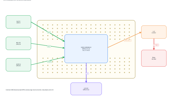
Fig. 3. ESP32 breadboard with sensors and relay module.
