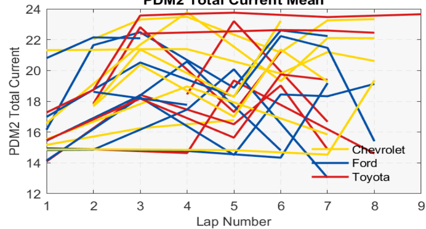
PDM2 Total Current Mean
