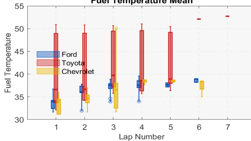
Fuel Temperature Mean
