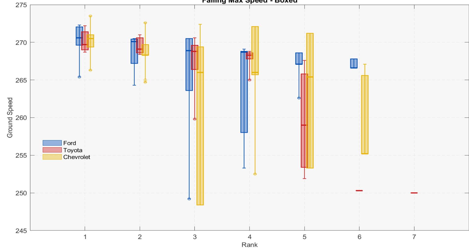
Falling Max Speed - Boxed
