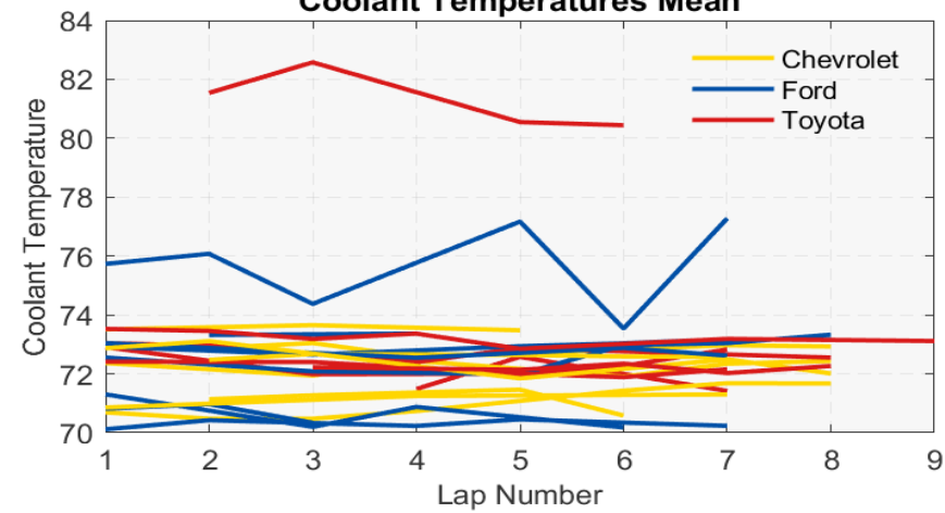
Coolant Temperature Mean
