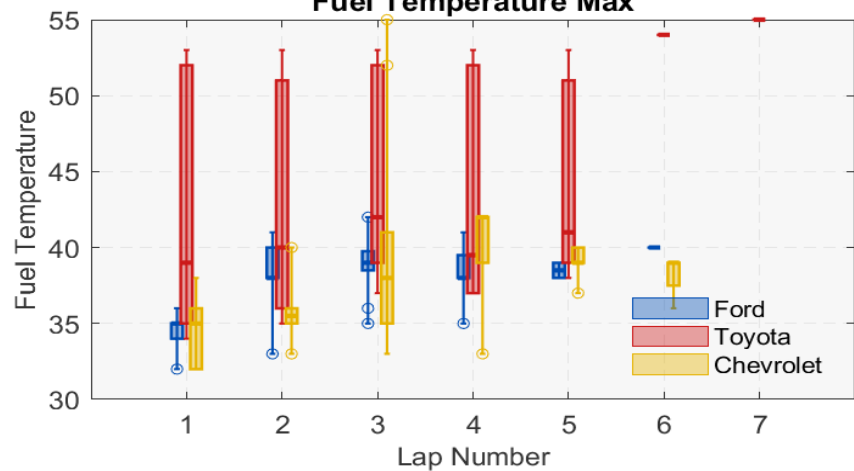
Fuel Temperature Max
