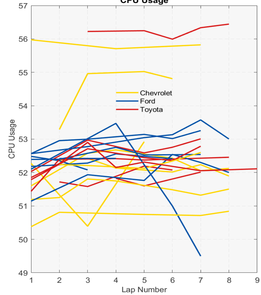
CPU Usage
