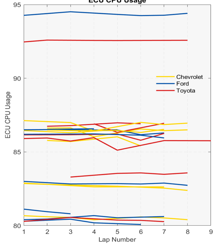
ECU CPU Usage
