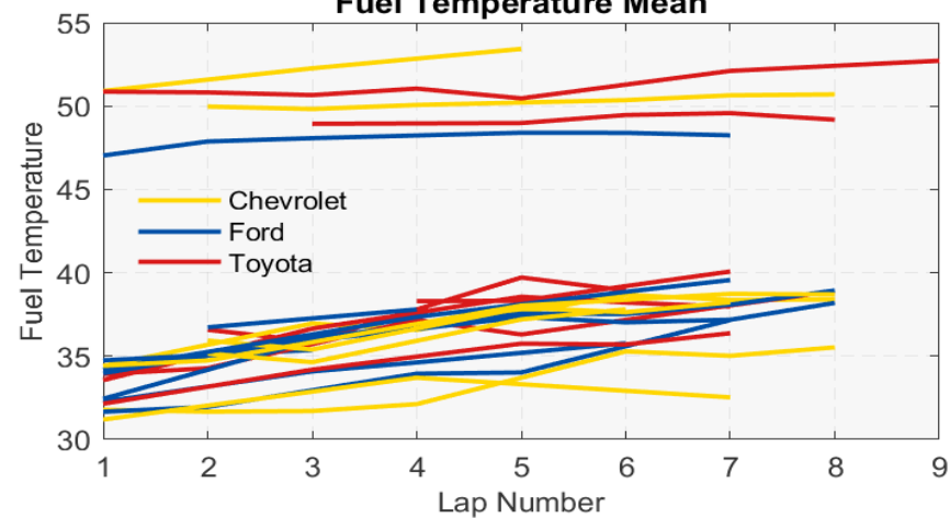
Fuel Temperature Mean
