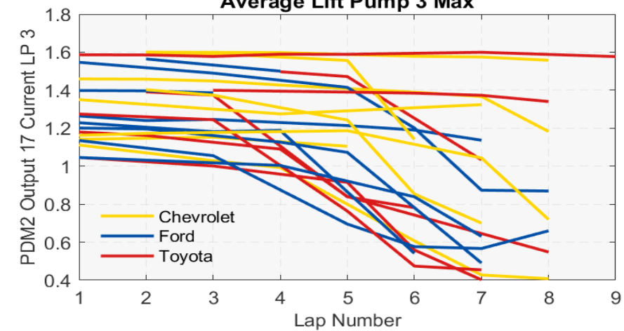
Average Lift Pump 3 Max
