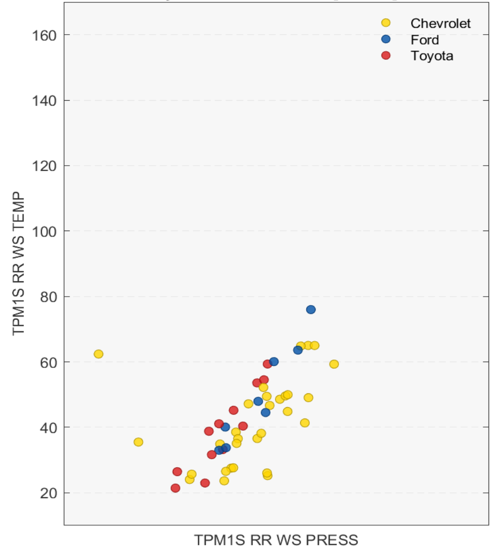
Tyre Performance RR [kPa/°C]
