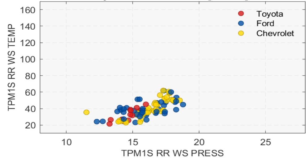
Tyre Performance RR [kPa/°C]
