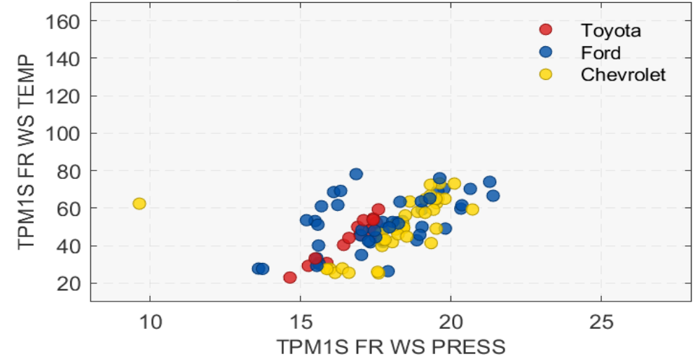
Tyre Performance FR [kPa/°C]
