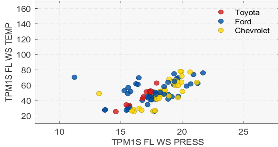
Tyre Performance FL [kPa/°C]
