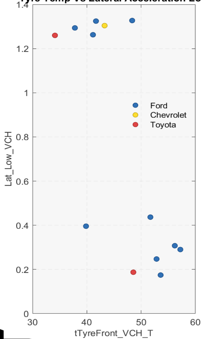
Tyre Temp Vs Lateral Acceleration Low
