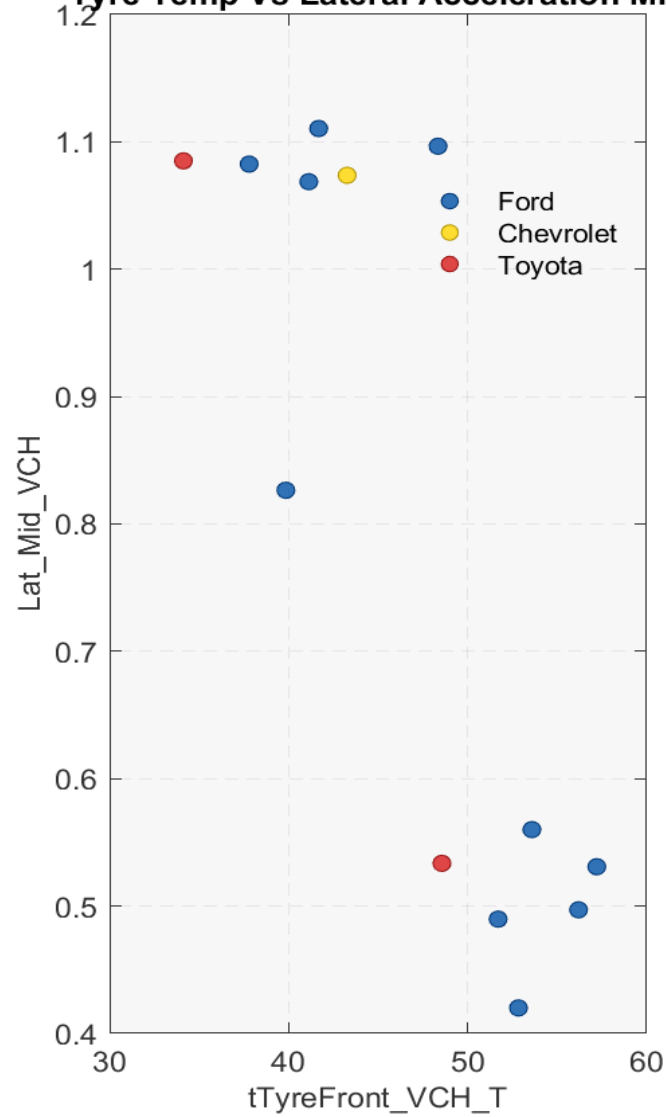
Tyre Temp Vs Lateral Acceleration Mid
