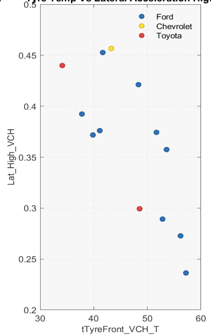
Tyre Temp Vs Lateral Acceleration High
