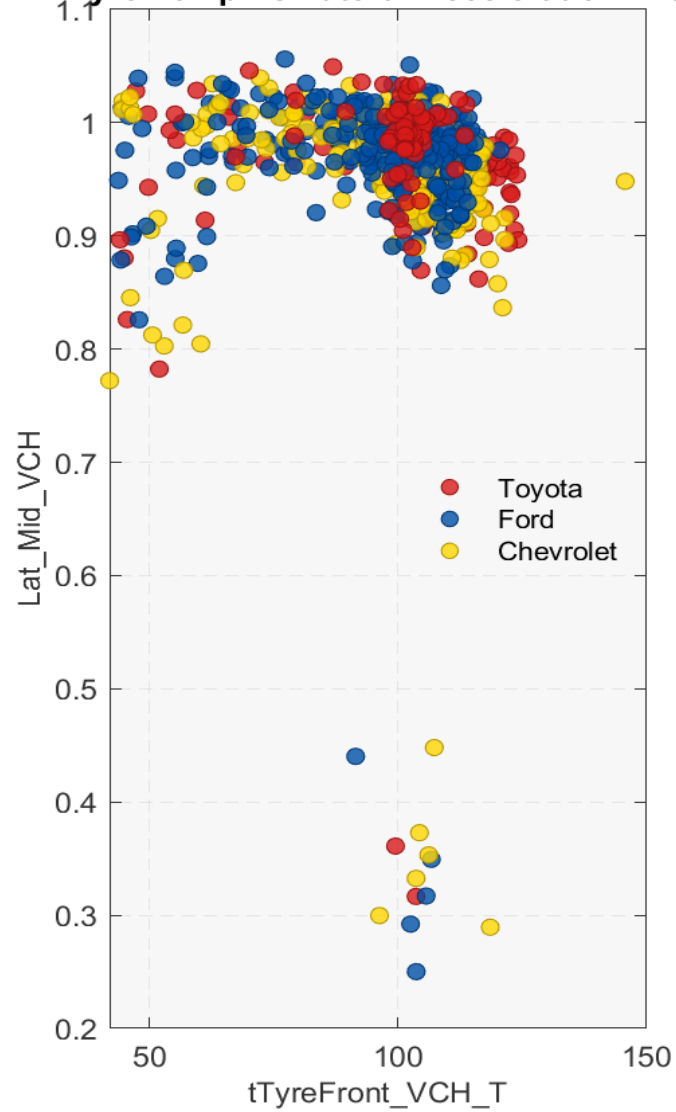
Tyre Temp Vs Lateral Acceleration Mid
