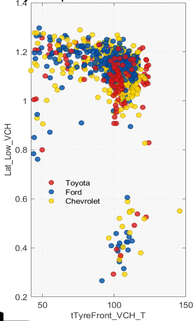
Tyre Temp Vs Lateral Acceleration Low
