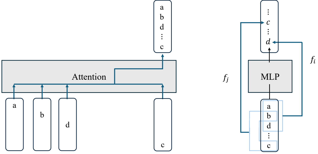
Figure 9. Illustration of the role of the attention and feedforward layers in looped TFs for evaluating DAGs: the attention layer uniformly attends to and aggregates all inputs at each position, while the feedforward layer simultaneously simulates the functions of the nodes.
