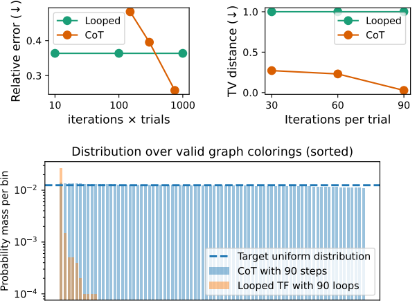
Figure 7. Top: Relative error for counting (left) and TV distance to uniform over valid colorings for sampling (right). Bottom: Empirical distributions for approximate sampling of graph colorings.
