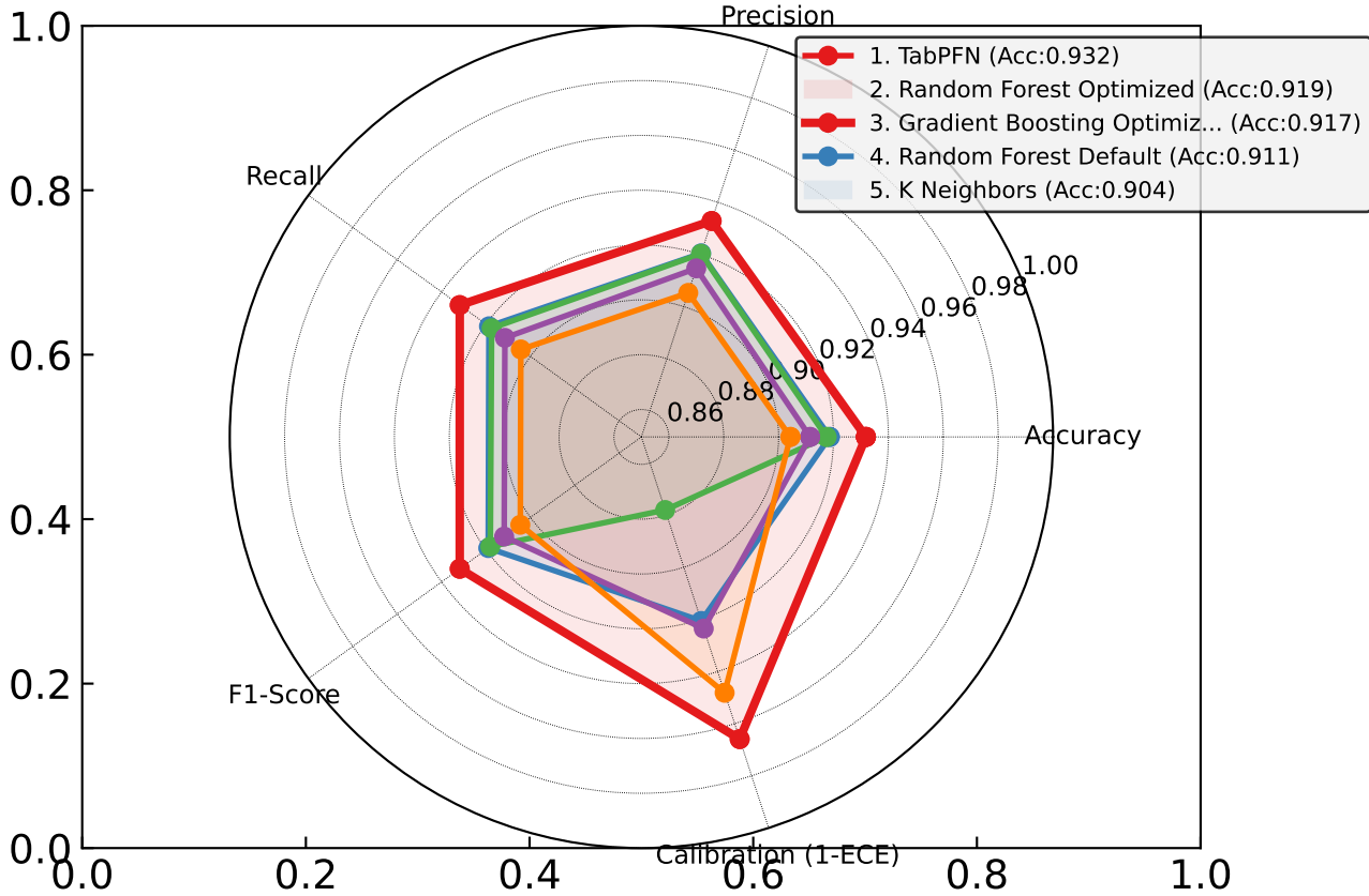
Top 5 Models - Metrics Comparison
