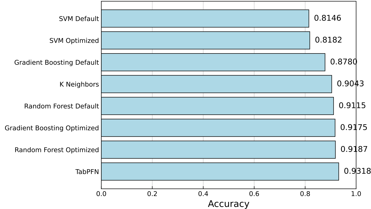
Accuracy Comparison - All Classification Models
