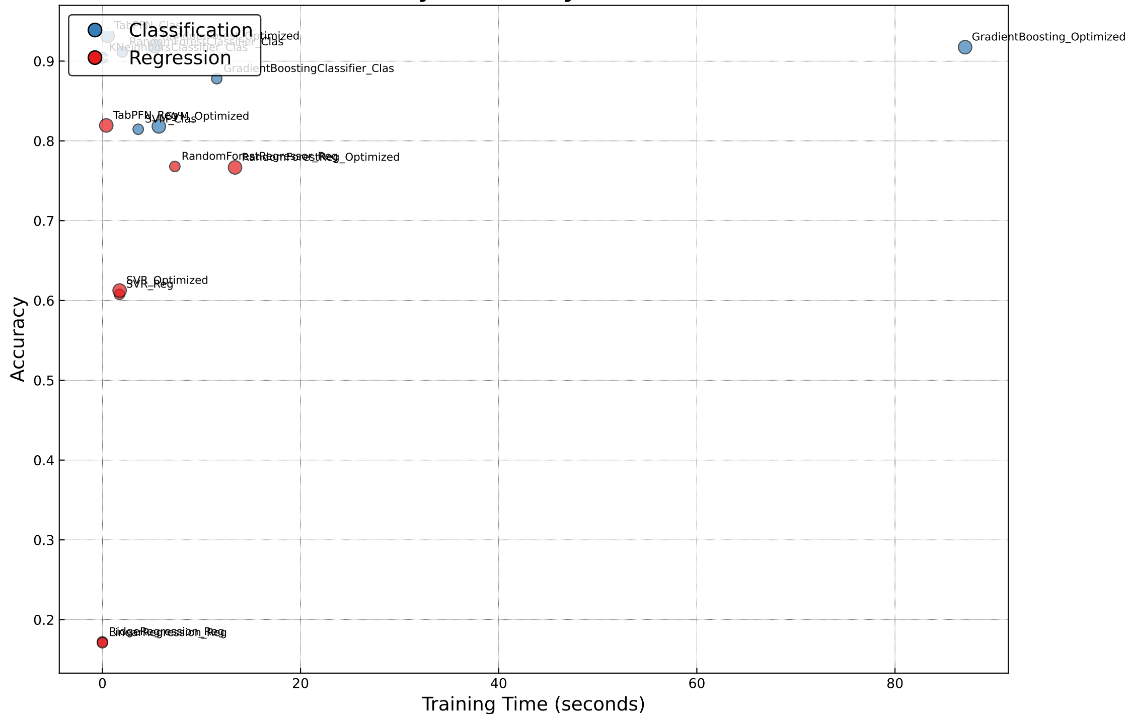
Time-Accuracy Tradeoff by Model - Mar Menor
