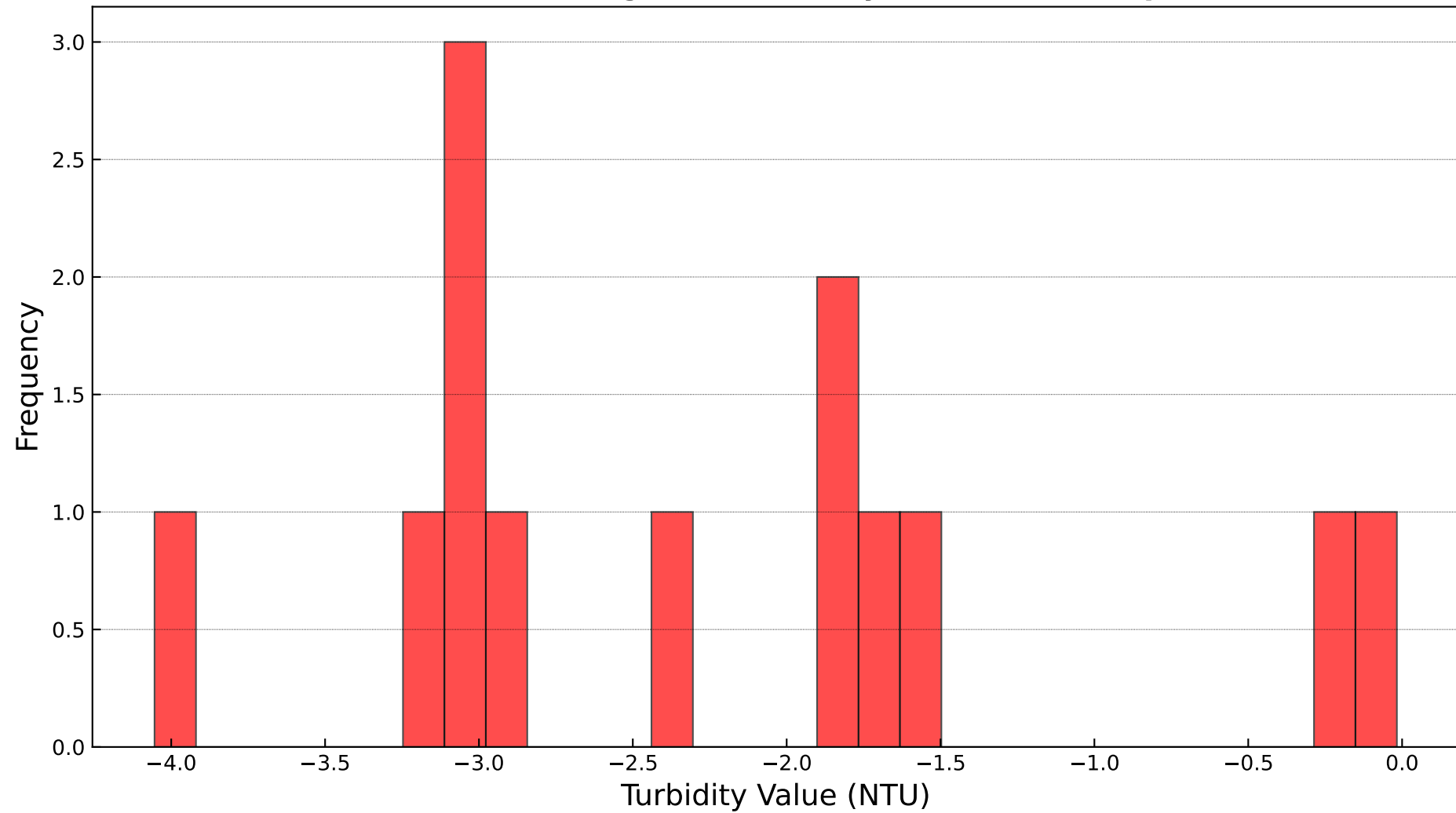
Distribution of Negative Turbidity Values (13 samples)
