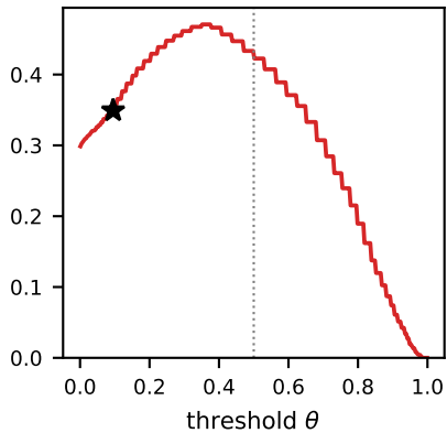
SVD JS
