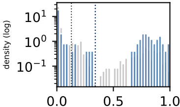
TwinSFT-noSplits (gap 0.21)
