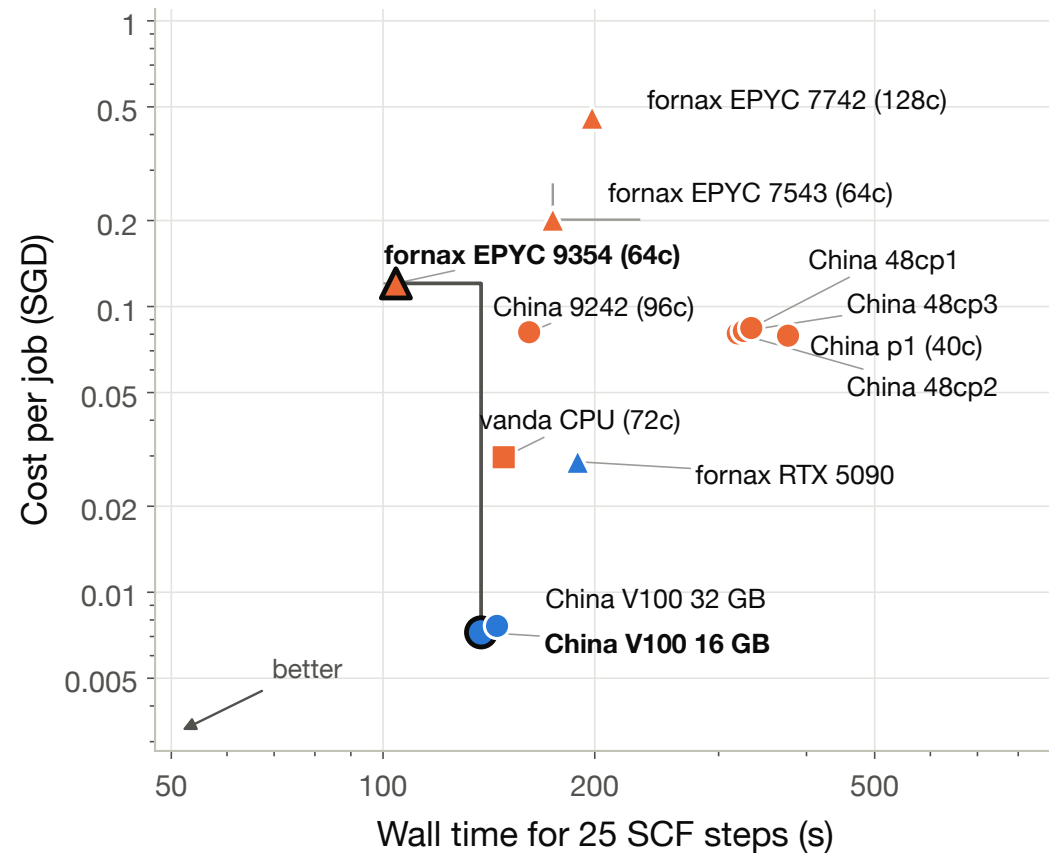
(a) VASP 6.5.1 — Na 3 PS 4 , 128 atoms, 25 SCF steps
