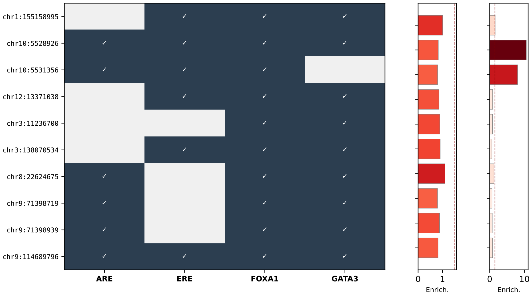
TF Motif Presence (HOMER scans)
