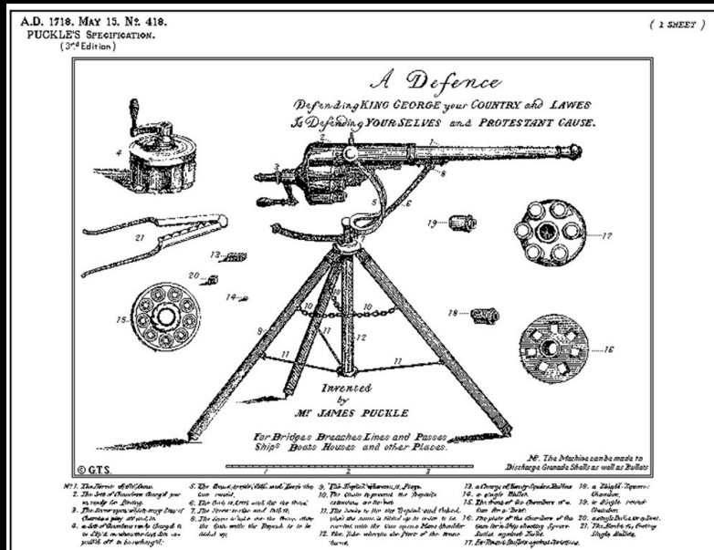
From James Puckle's 1718 early autocannon patent
