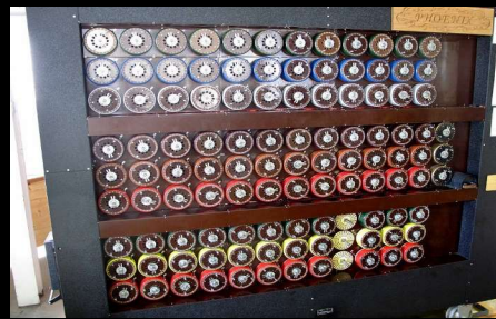
Turingbombe
