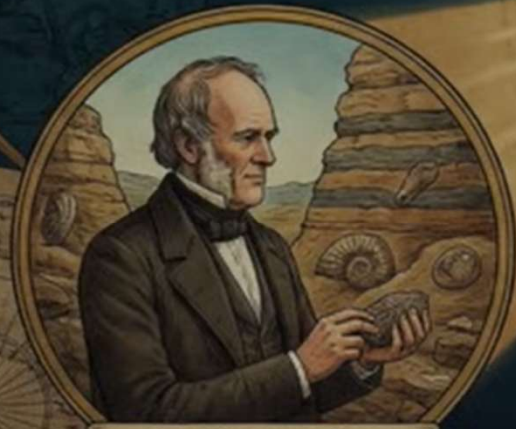
Earth's Deep Time
