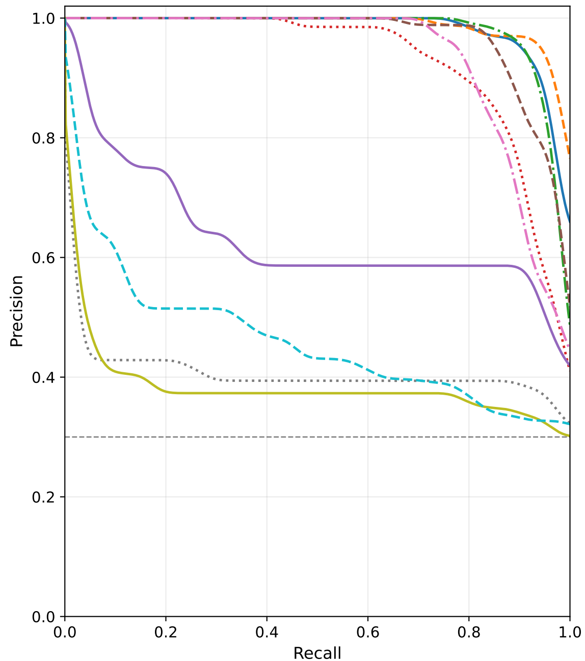
(a) Precision-Recall
