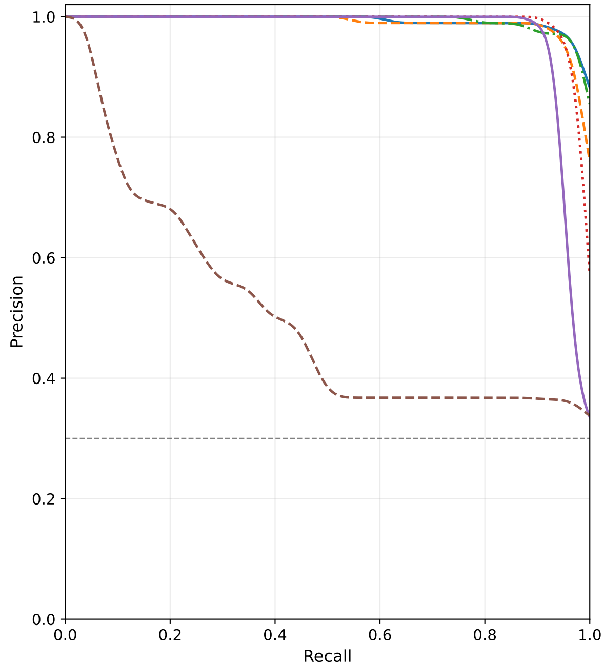
(a) Precision-Recall
