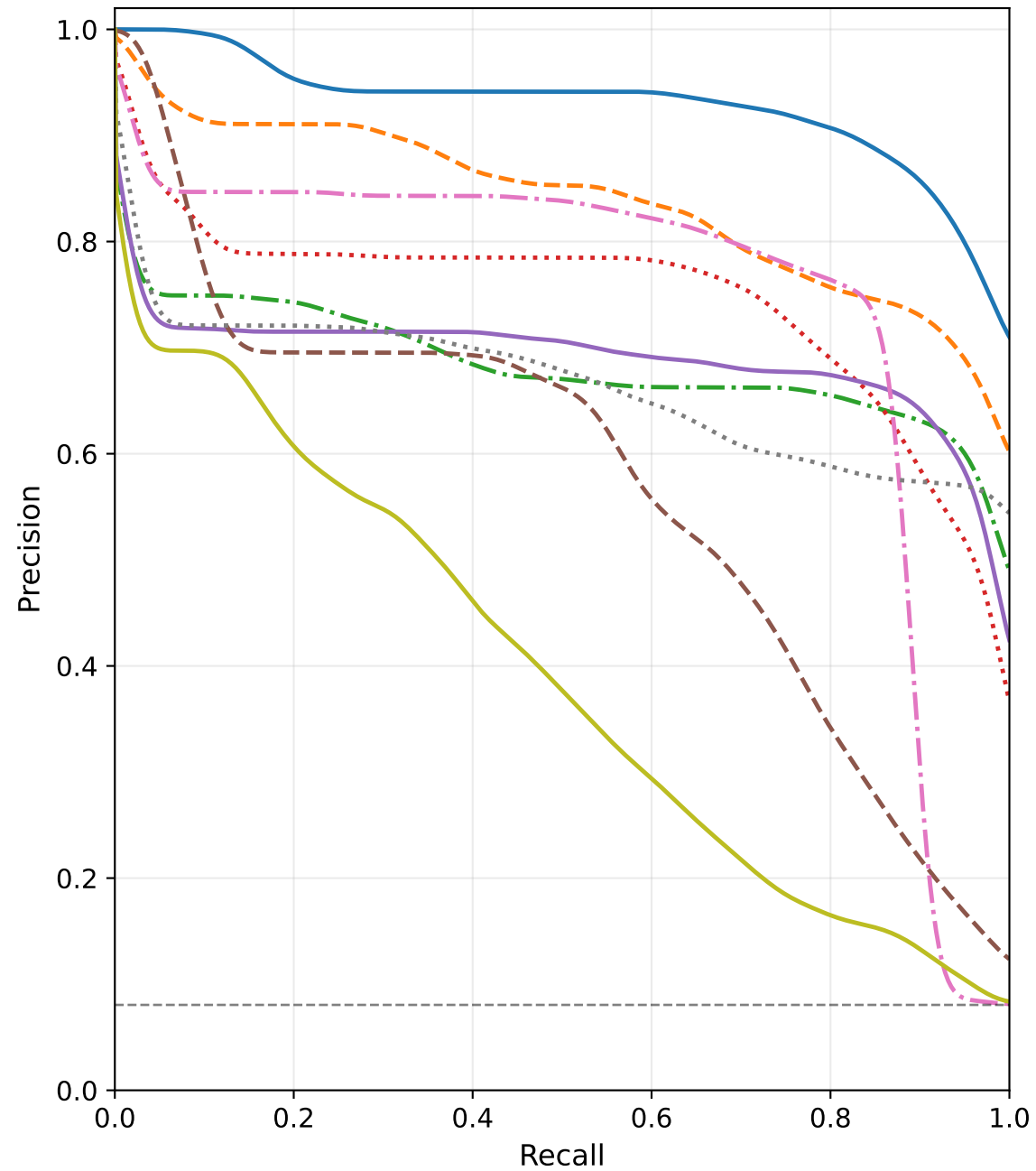
(a) Precision-Recall
