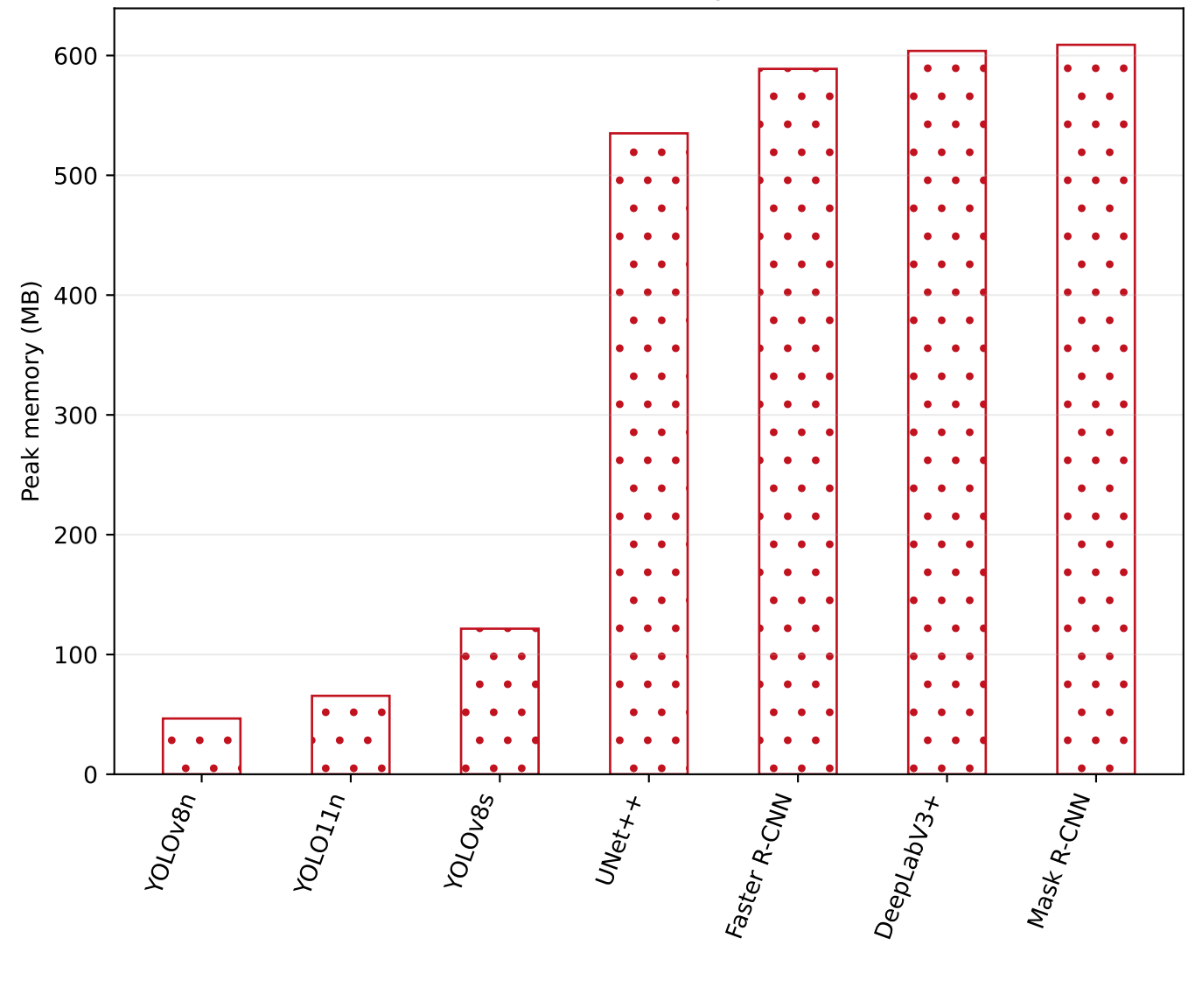
(b) Peak memory, GPU
