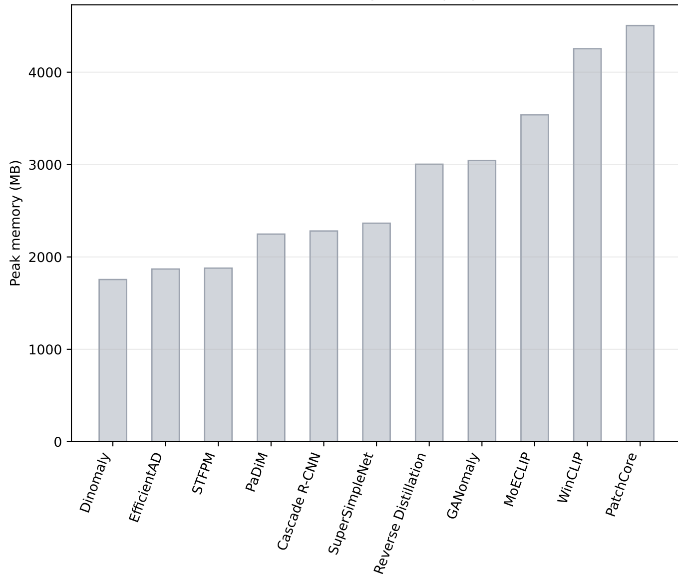
(a) Peak memory, whole program
