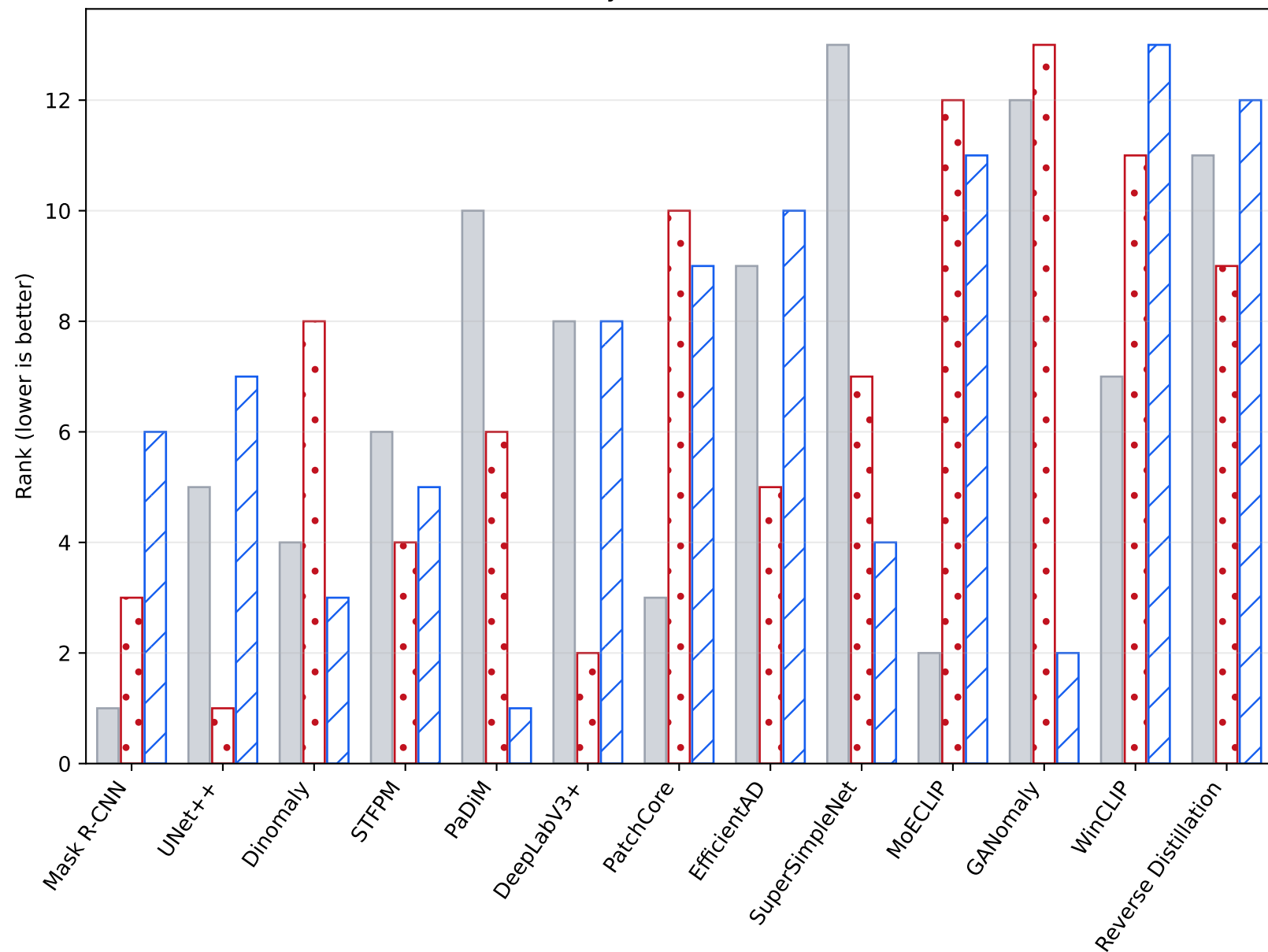
(a) Anomaly detection / zero-shot
