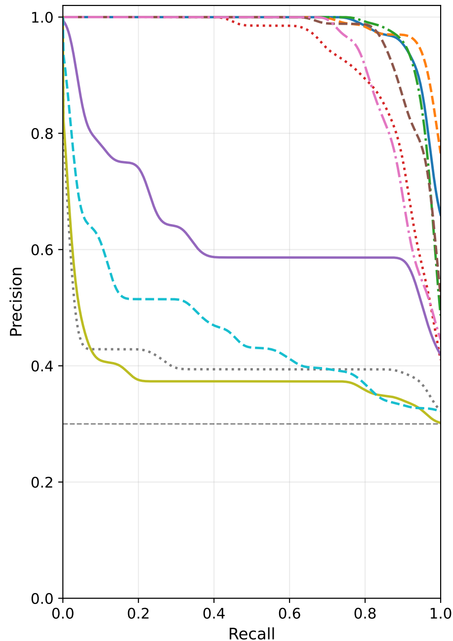
(a) Precision-Recall
