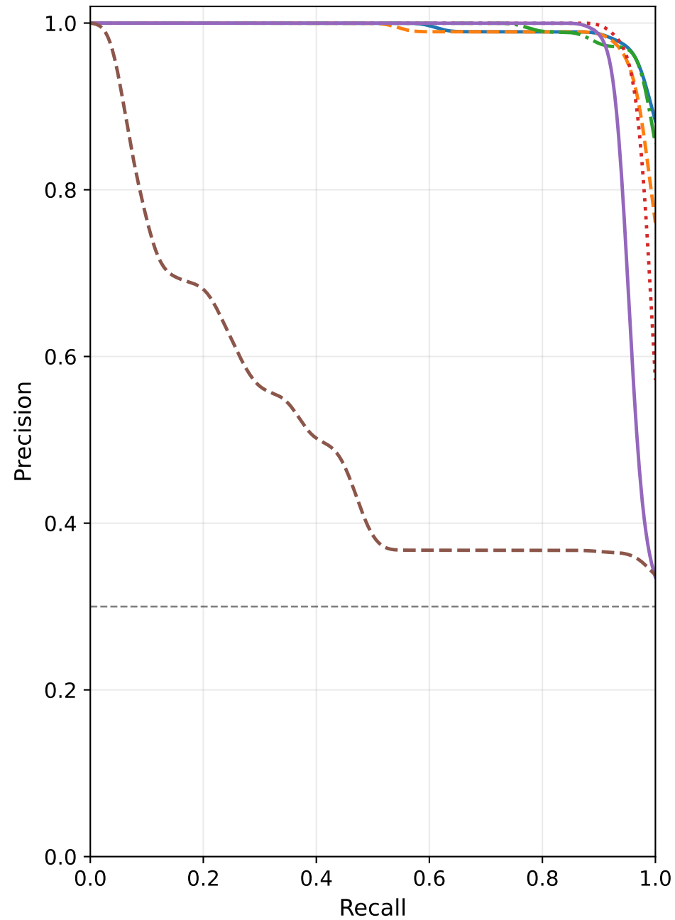
(a) Precision-Recall
