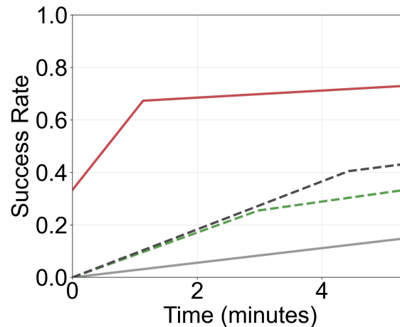
(b) Dexterous hand Baselines / VLASelect avg. acc: 0.3833 / 0.7639 (38.06%↑)
