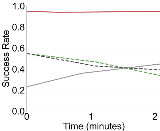
(a) Single-arm robot Baselines / VLASelect avg. acc: 0.4200 / 0.8982 (47.82%↑)
