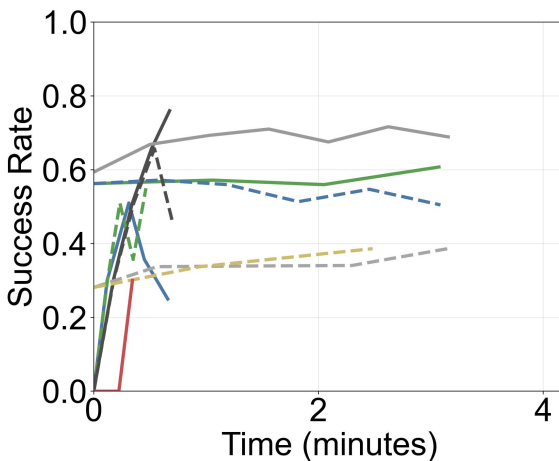
(a) Single-arm robot Baselines / VLASelect avg. acc: 0.5596 / 0.2500 (-30.96% \uparrow )
