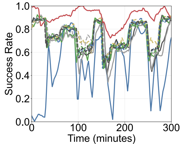
(b) Dexterous hand Baselines / VLASelect avg. acc: 0.6540 / 0.8233 (16.93%↑)
