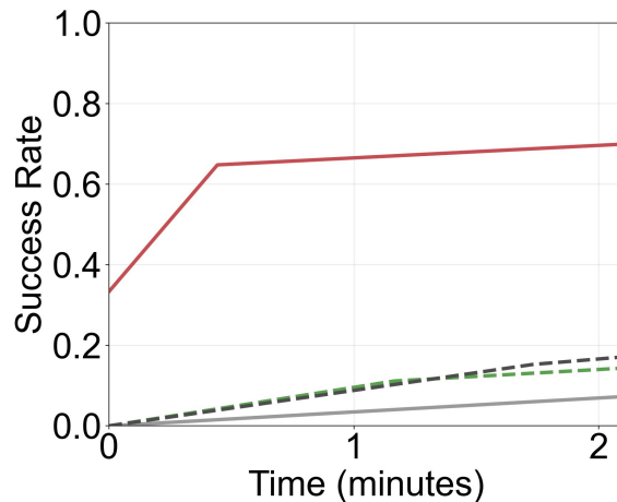
(b) Dexterous hand Baselines / VLASelect avg. acc: 0.1623 / 0.7306 (56.82%↑)
