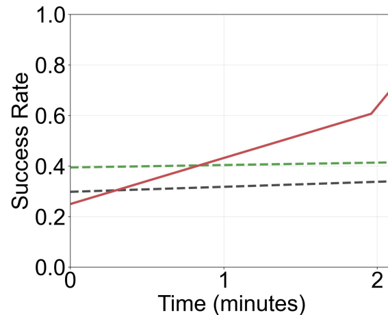
(c) Mobile manipulator Baselines / VLASelect avg. acc: 0.3755 / 0.7750 (39.95%↑)
