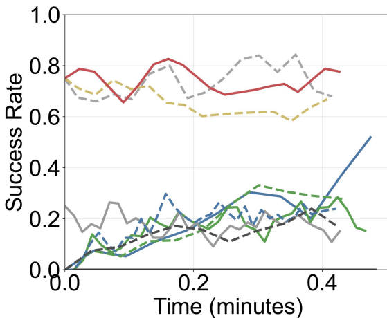
(a) Single-arm robot Baselines / VLASelect avg. acc: 0.2942 / 0.7500 (45.58%↑)
