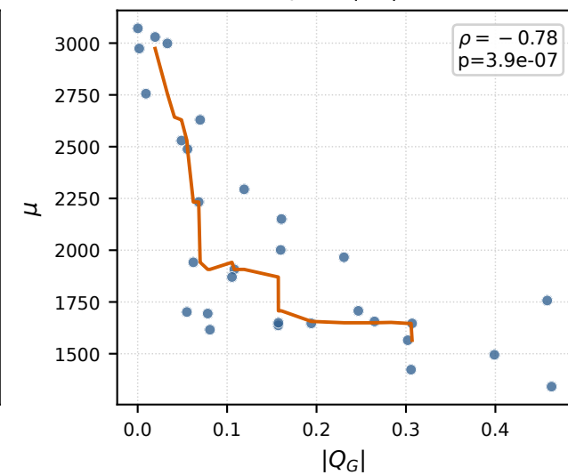
\mu vs. |Q_G|
