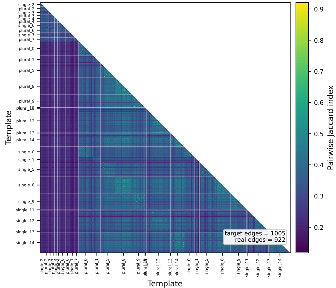
Template-dependent sample circuits for GPT-2 small on SVA
