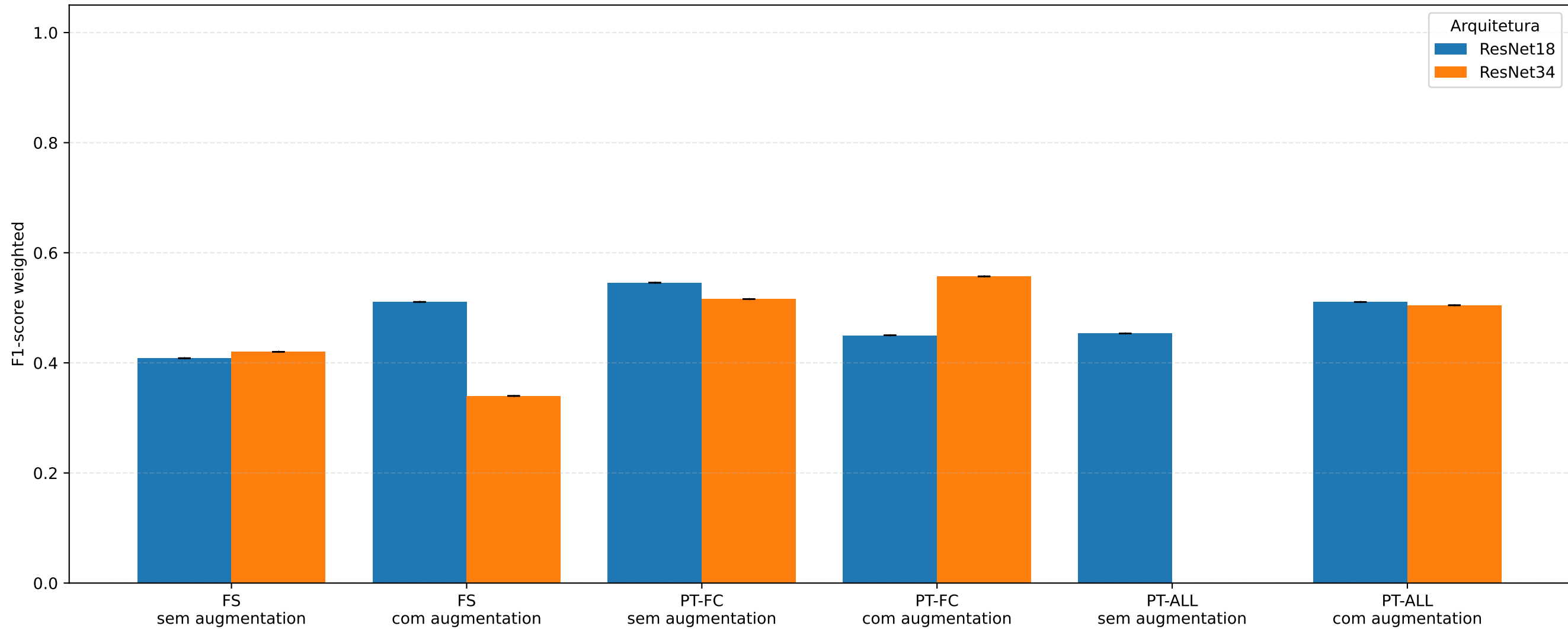
F1-score weighted global - ndb
