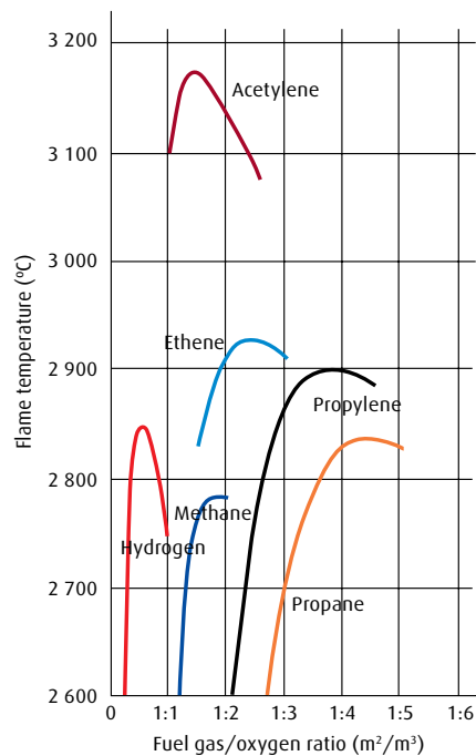
Flame temperatures fuel gas/oxygen
