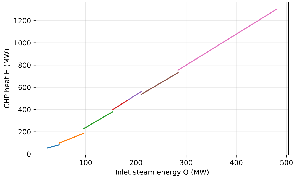
Heat segments (H-Q), temp=75C
