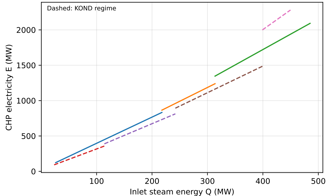
Power segments (E-Q), temp=75C
