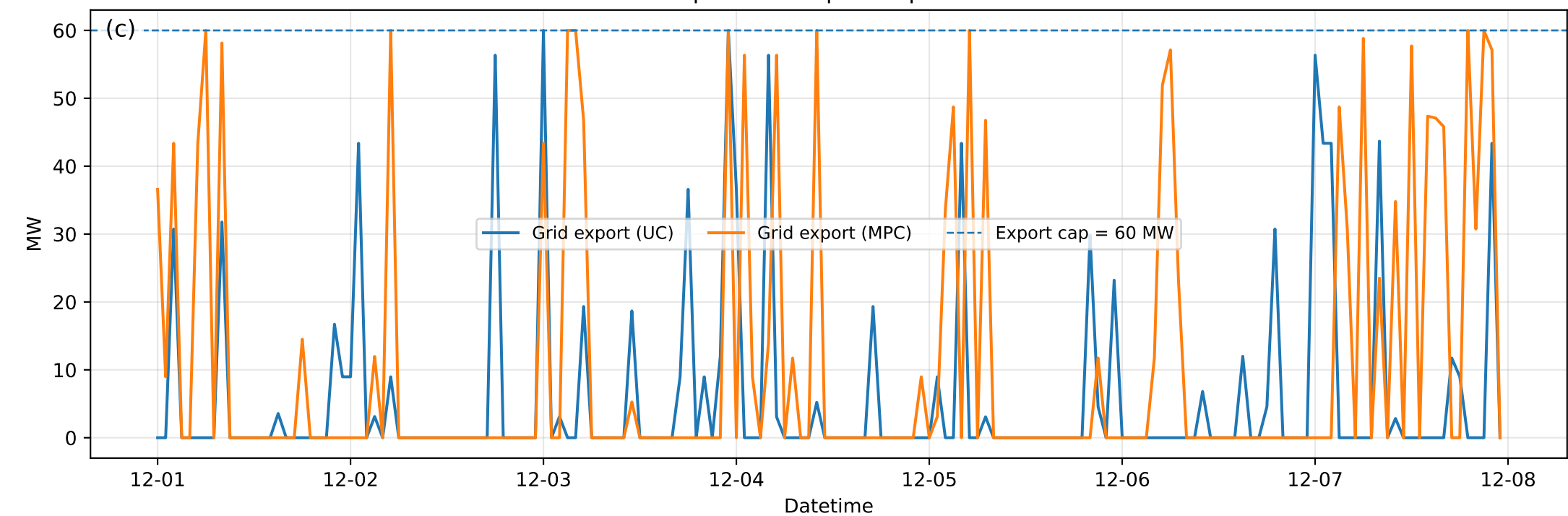
Grid export and export-cap saturation
