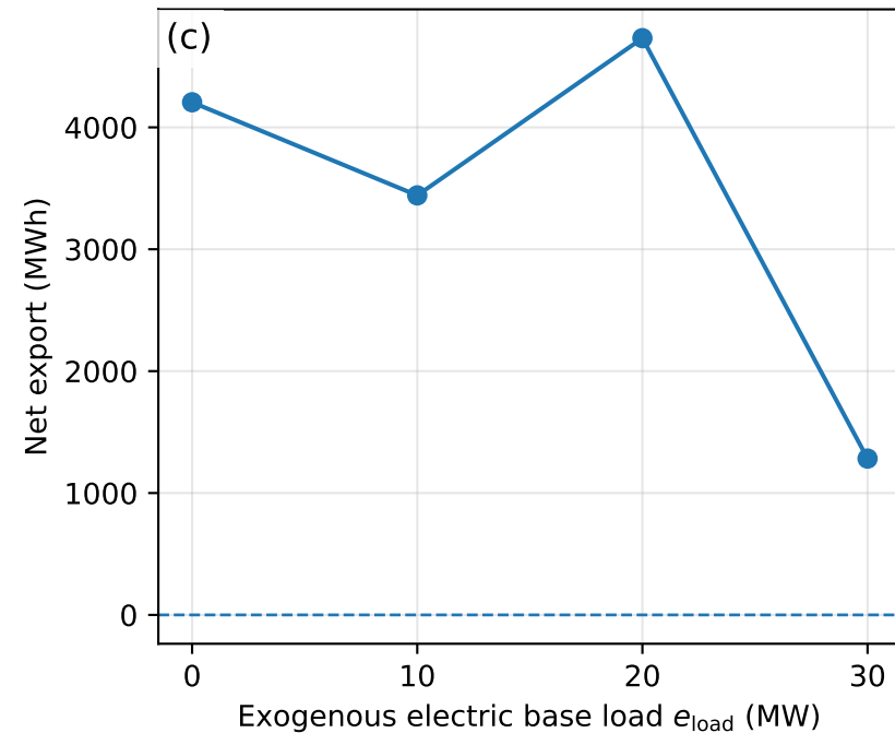
Net grid export
