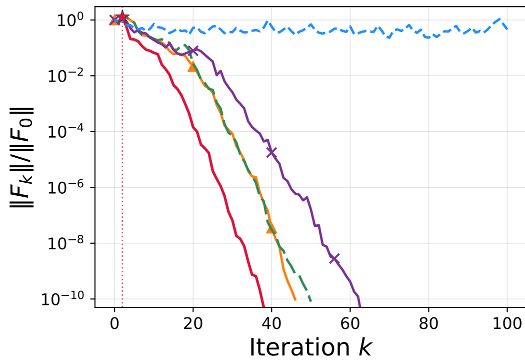
DOFs=2,118, Re = 5000
