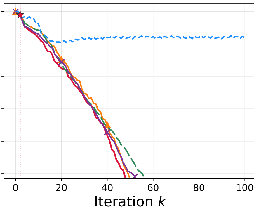
DOFs=48,422, Re = 8000
