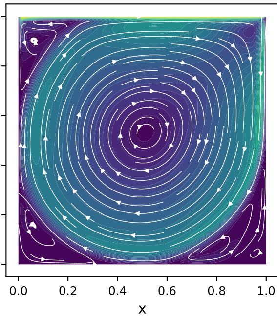
DOFs=48,422, Re = 8000 GlobAA(50)
