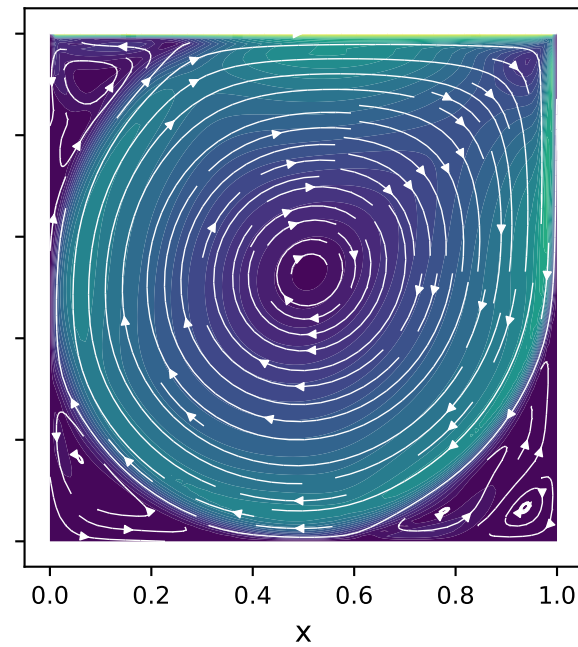
DOFs=190,542, Re = 10000 GlobAA(50)
