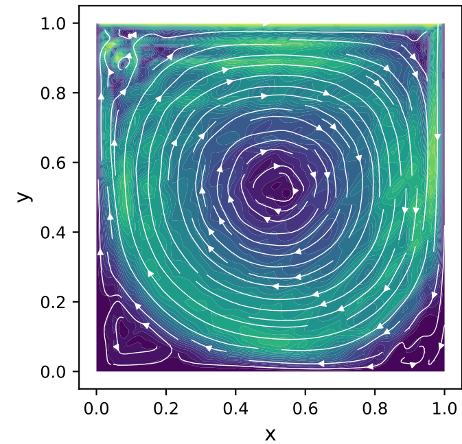
DOFs=2,118, Re = 5000 GlobAA(50)
