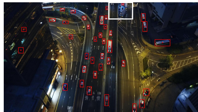
Result (Baseline)
