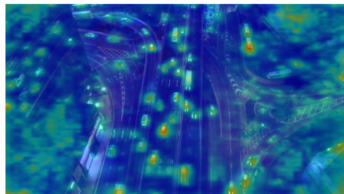
Heatmaps (Baseline)
