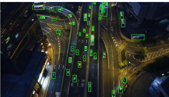
GT
