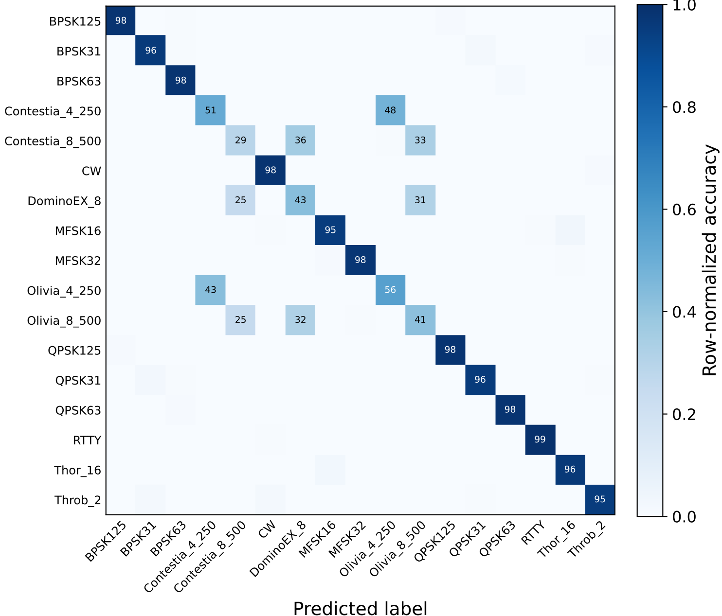
Normalized confusion matrix: Conformer
