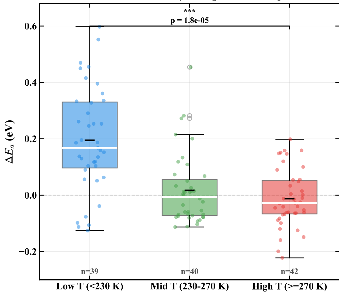
(c) \Delta E_a Distribution by Temperature Region
